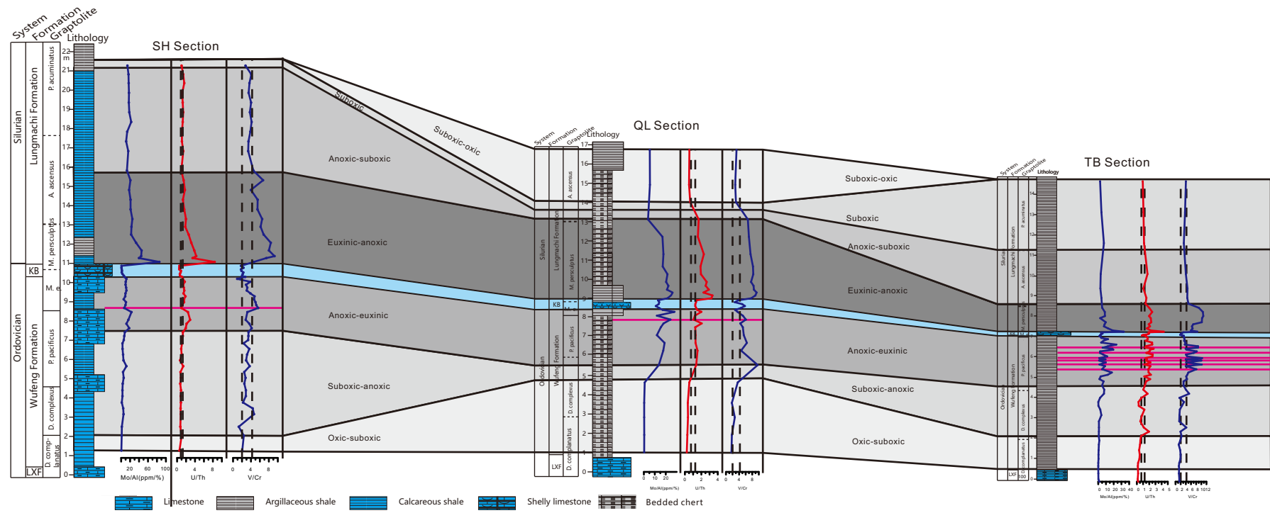
Figure S2. Stratigraphic correlation of redox conditions proxies. Dashed lines from low to high values show the trends of redox changes. (Mo, U and V data cited from Zou et al., 2018a).
